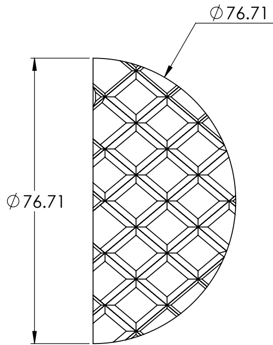
TOP VIEW
