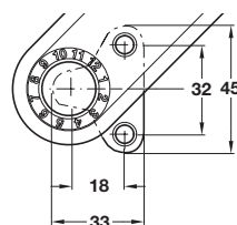
Screw-on bracket for fixing to the carcase side panel
