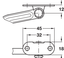
Angled foot bracket for fixing to flaps made of wood
